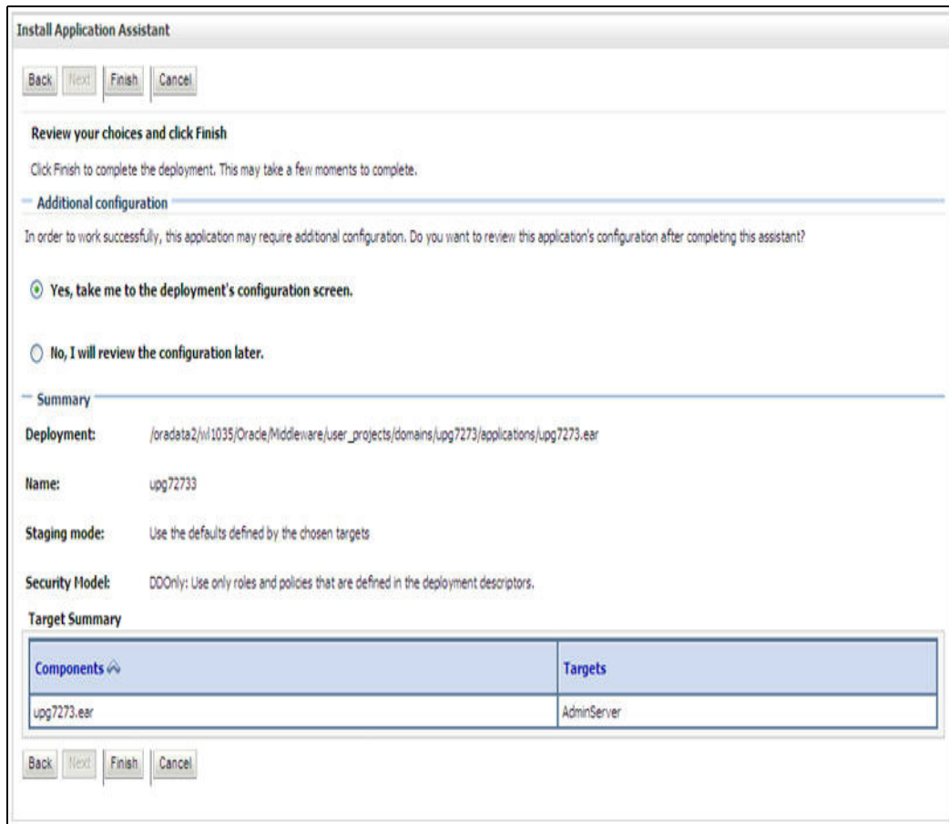
Figure 6–53 Deployment Summary
