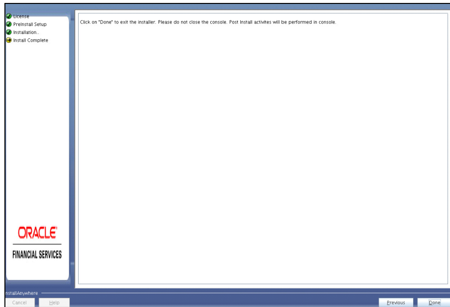
Figure 4–32 Installation Complete
