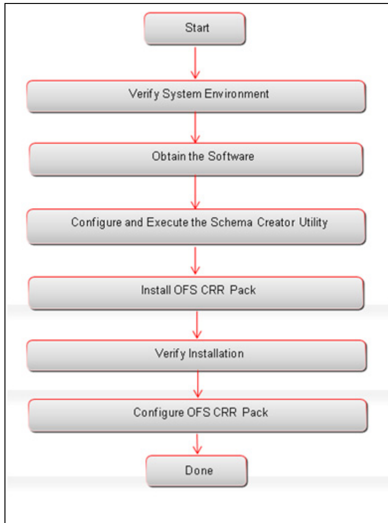
Figure 2–1 Installation Overview
