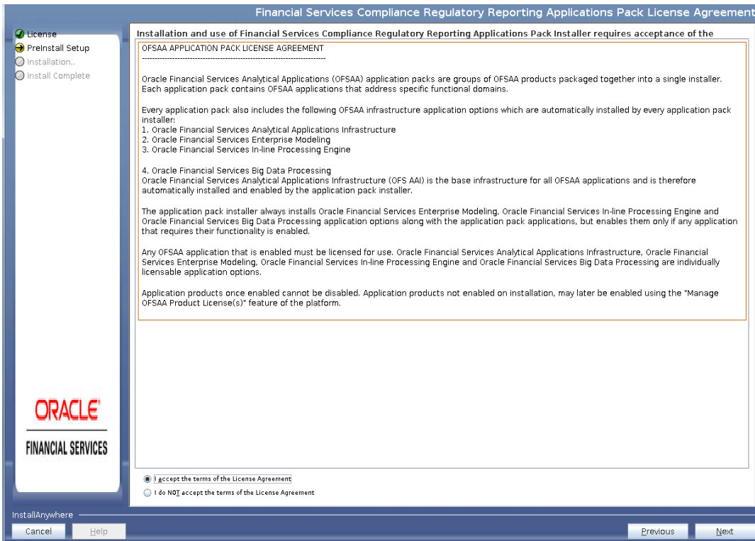
Figure 4–8 License Page
