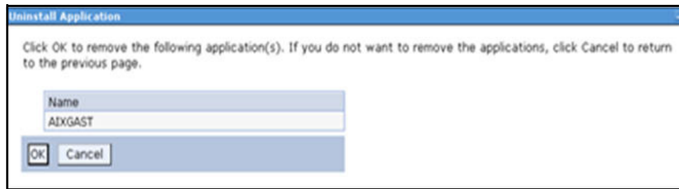
Figure 6–61 Uninstall Application
