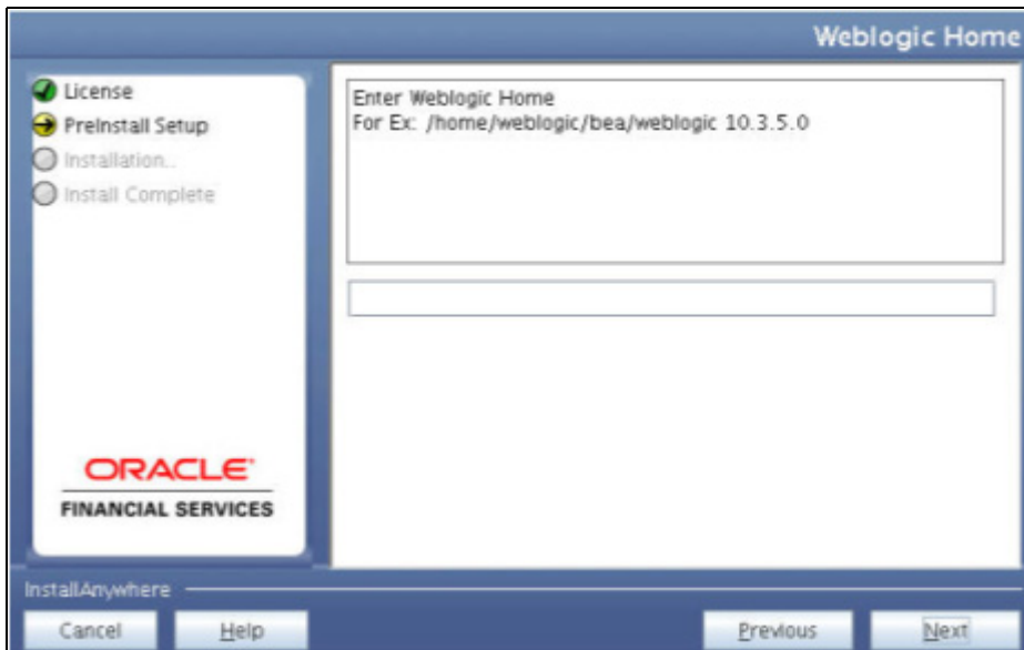
Figure 4–18 Weblogic Home
