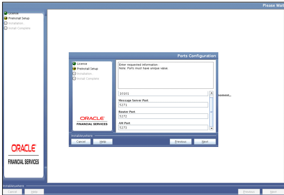
Figure 4–24 Ports Configuration
