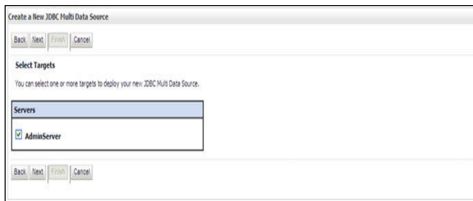
Figure 6–35 Select Targets
