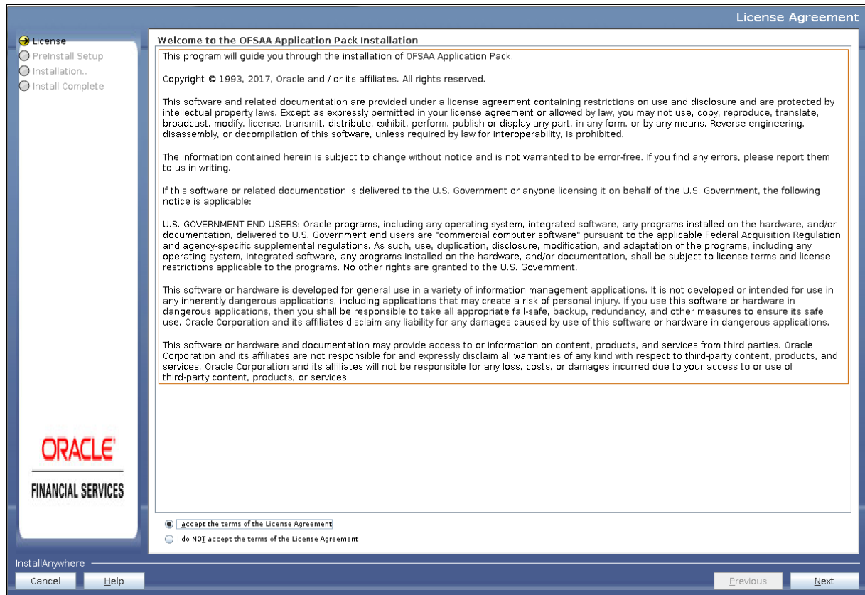
Figure 4–5 License Agreement
