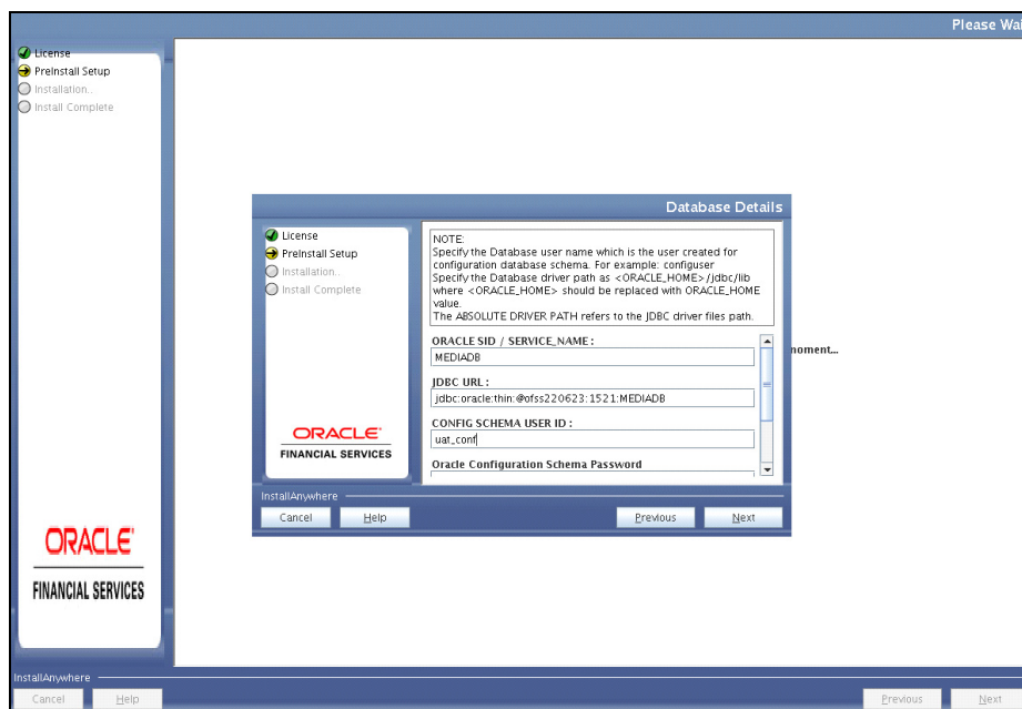
Figure 4–22 Database Details
