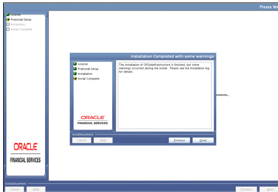
Figure 4–30 Installation Complete
