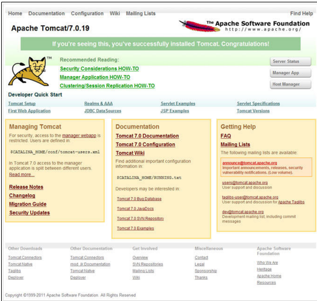
Figure 6-57 Tomcat home
