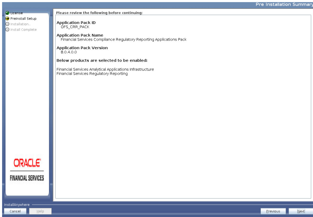
Figure 4–9 Pre-installation Summary
