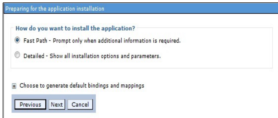
Figure 6-42 Installation Options
