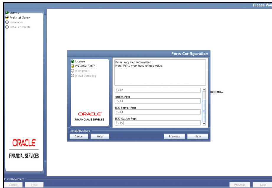
Figure 4–23 Ports Configuration
