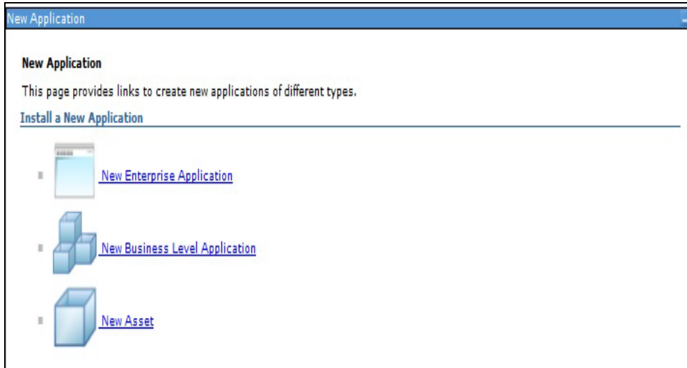
Figure 6–40 New Application
