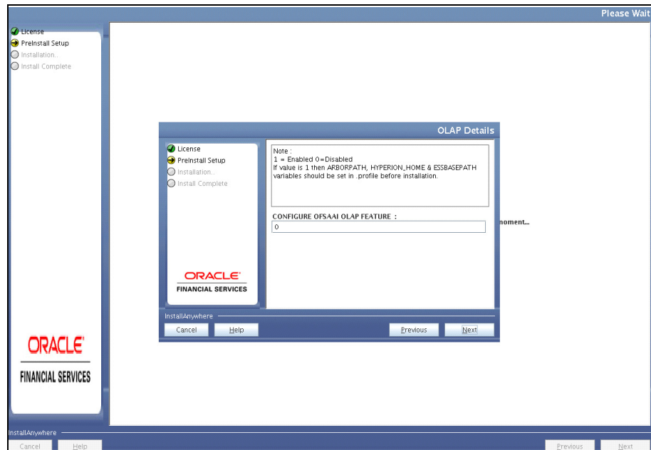
Figure 4–20 OLAP Details
