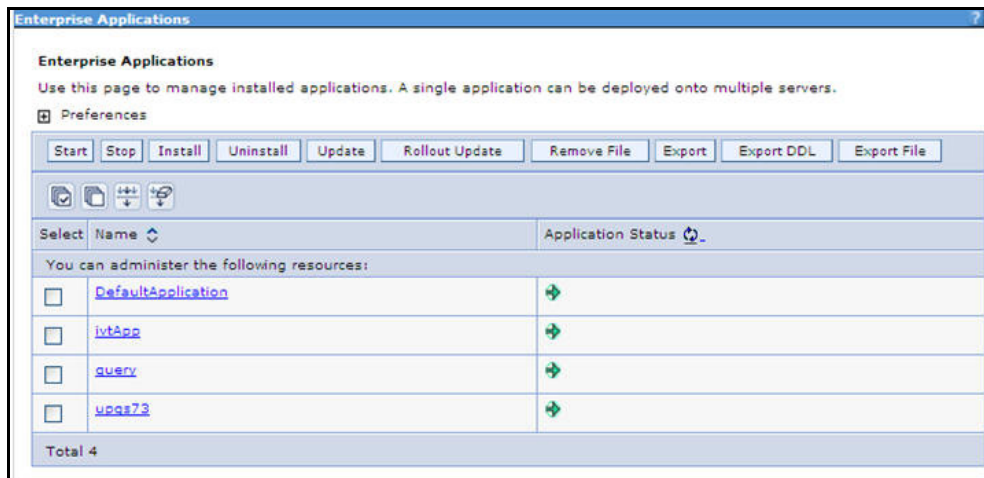
Figure 6–60 Enterprise Applications
