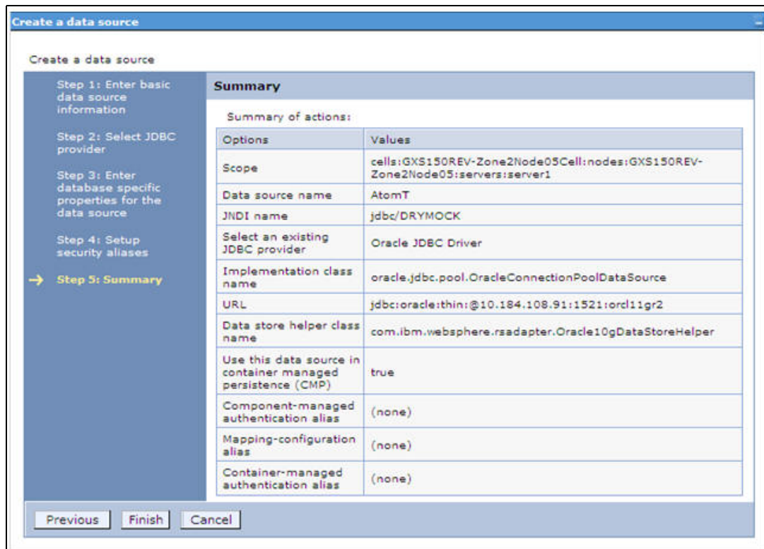
Figure 6–21 Summary
