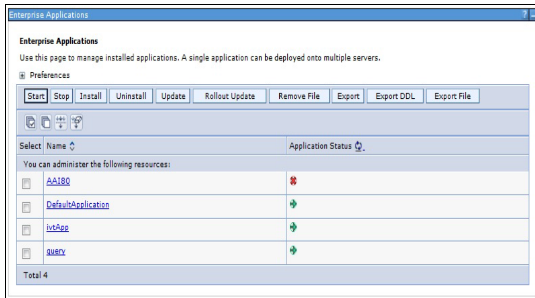
Figure 6-48 Enterprise Applications
