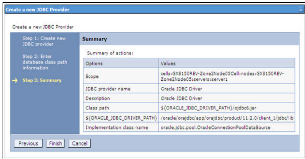
Figure 6–15 Summary
