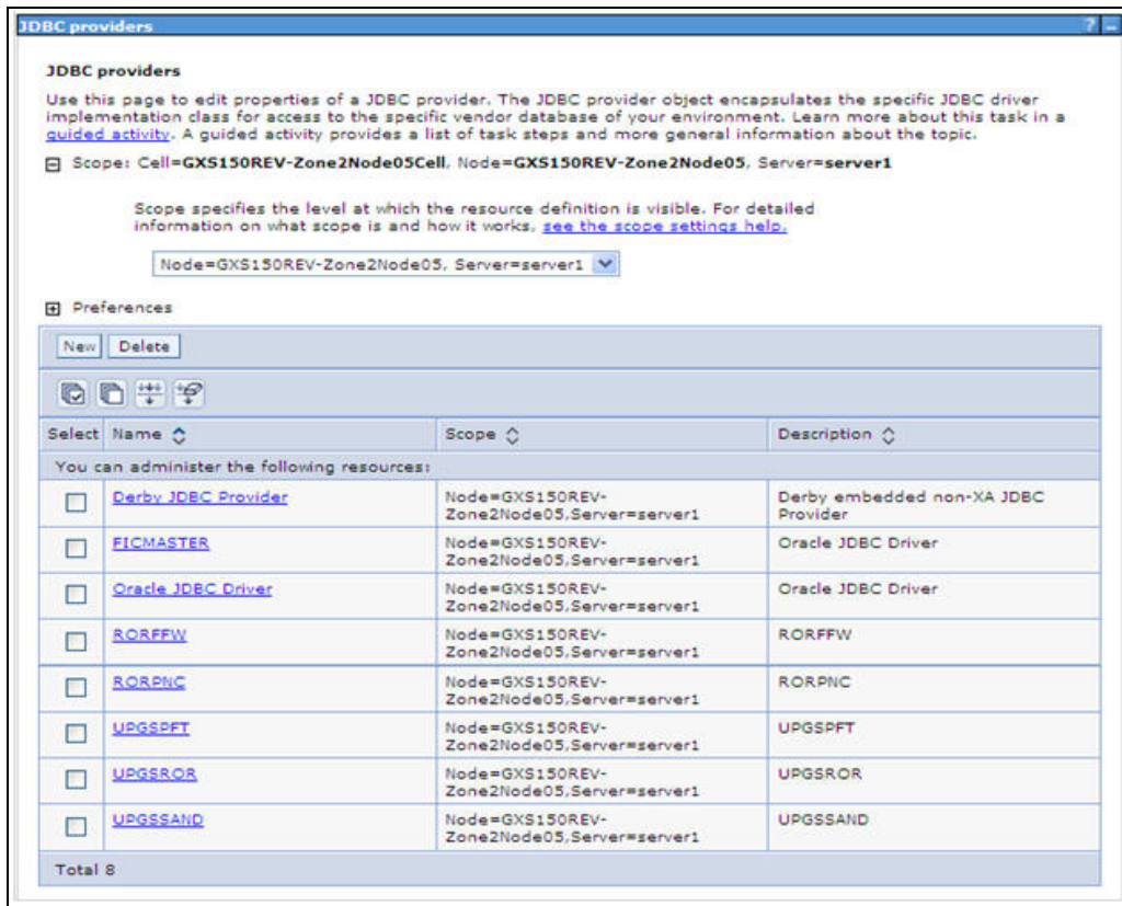
Figure 6–12 JDBC Providers
