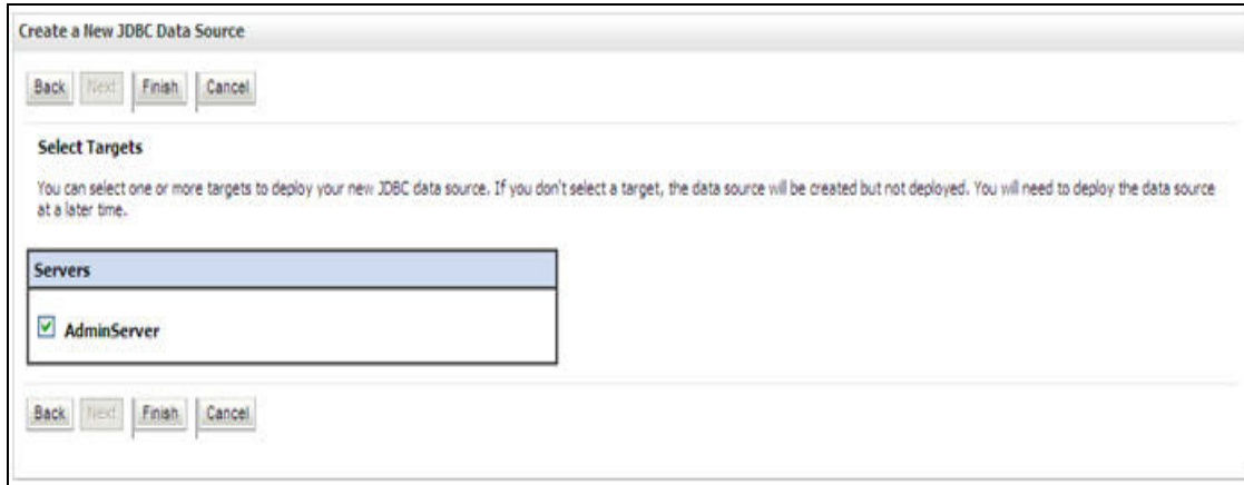
Figure 6–30 Select Targets
