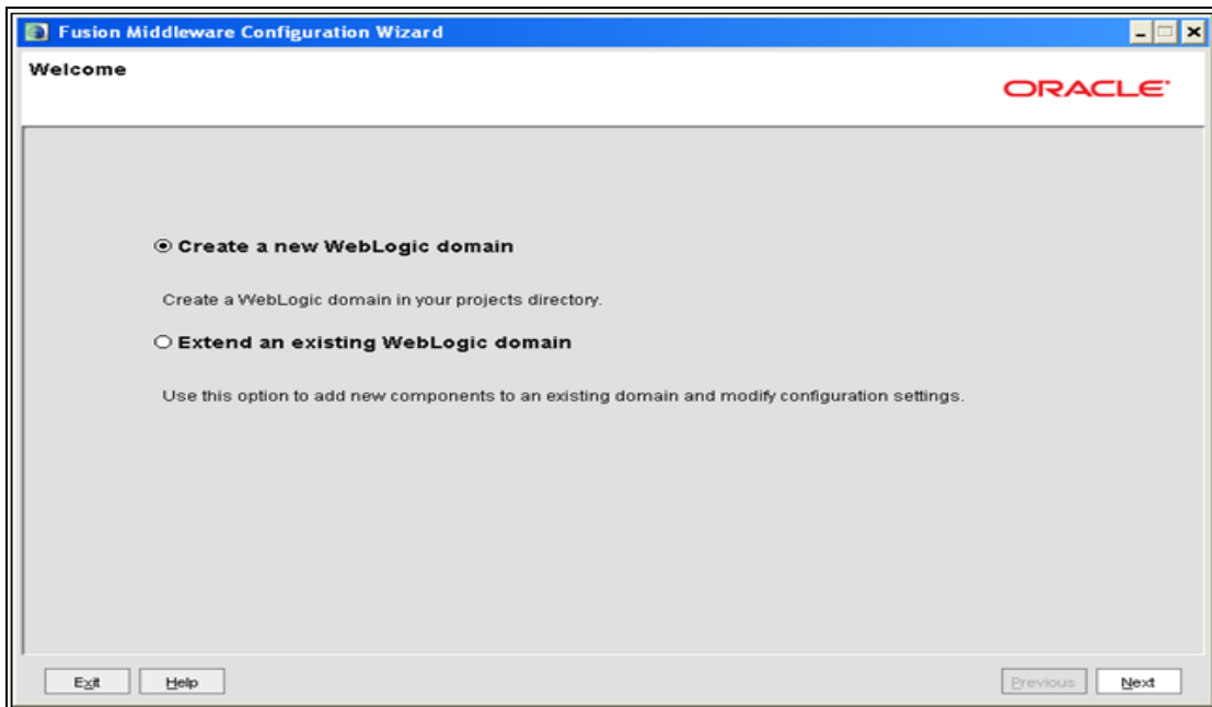
Figure 6–3 Welcome
