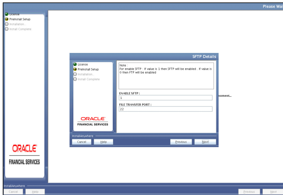
Figure 4–25 SFTP Details
